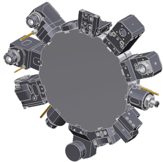
Abstechhalter cut-off holder
